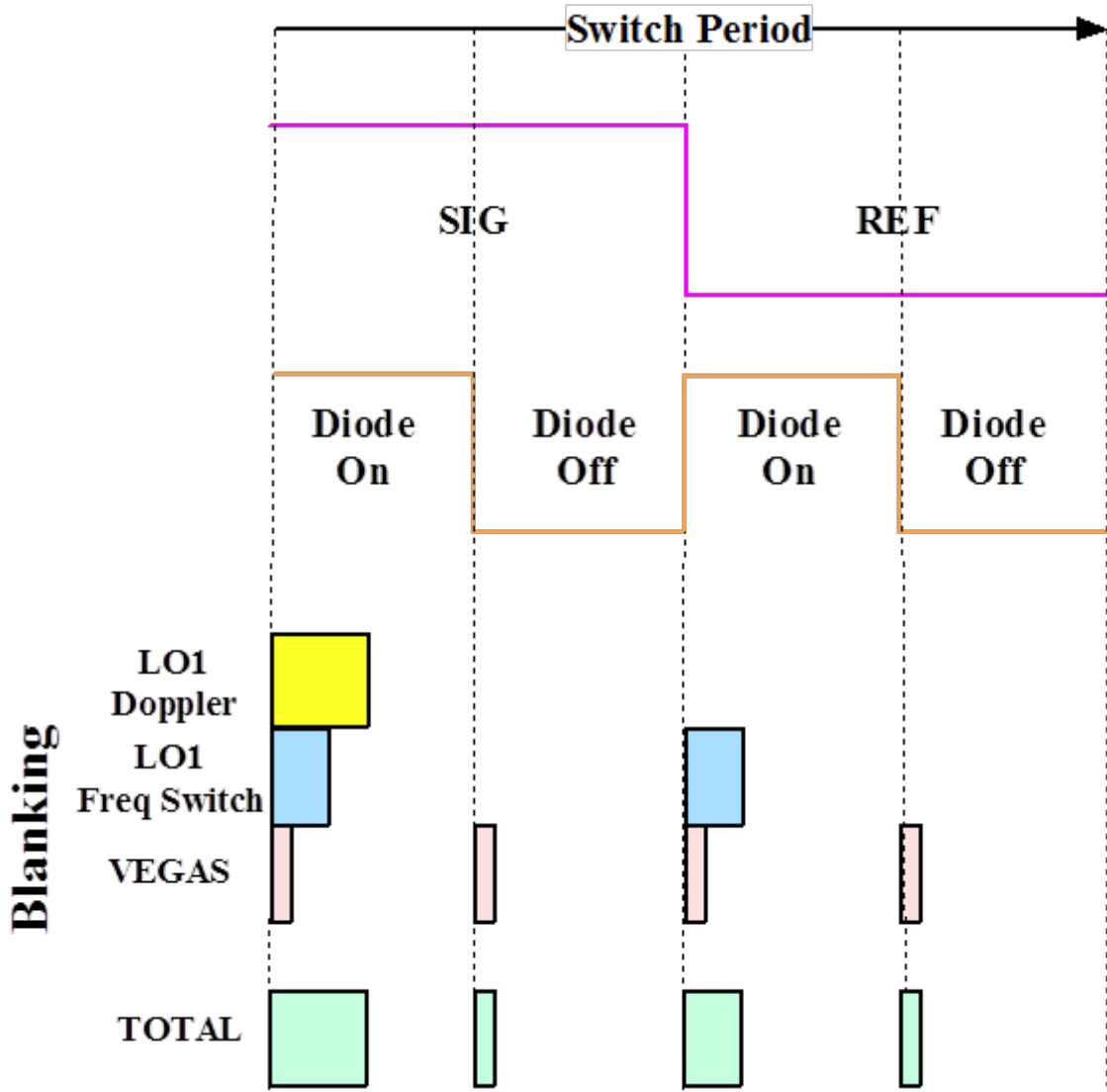
Figure 2: Blanking during frequency switched observations with the noise diode ( s_p ). The relative length of the LO blanking and minimum VEGAS blanking time vary depending on the VEGAS mode. For this example, we are assuming that the blanking interval from the LO due to the frequency switch is greater than the minimum blanking time for VEGAS. The magenta line shows the transition from the signal (sig) state to the reference (ref) state for the frequency switch and the orange line shows the noise diode turning on and off. The red boxes show the blanking introduced by VEGAS, which is triggered by state changes. The blue boxes are the blanking introduced by the LO due to frequency switching. The yellow box shows the blanking introduced by the LO while Doppler tracking. For frequency-switched observations, the Doppler tracking update always occurs in the first state of a switching period. The total blanking introduced on a state change is just the maximum of all the blanking values, not the sum.
