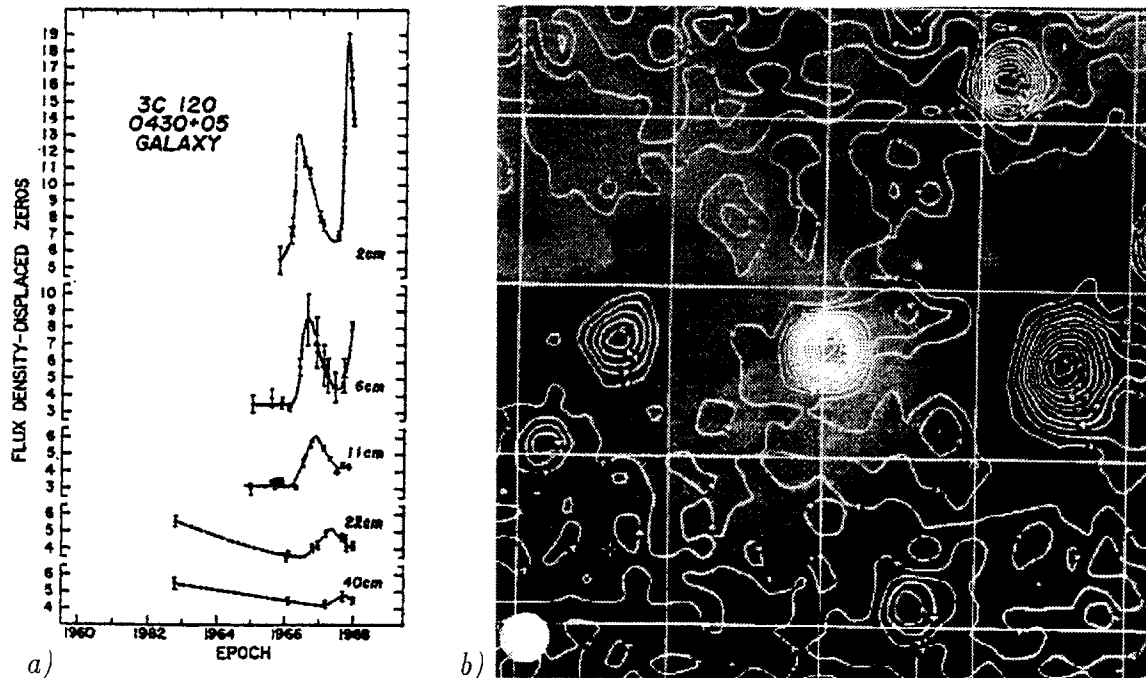
Figure 1: a) Variations of radio source flux density as a function of time and wavelength of observation (Kellermann and Pauliny-Toth 1968). Note much greater variation at 15 GHz (2 cm) than at lower frequencies. b) Radio wavelength image contours superimposed on a 1 square degree field containing the continuous gamma ray source L1688 (Schlickeiser et al. 1989, Astron. Astrophys. 216:197). Radio observations have been used to study star forming regions with gamma ray emission. The 15 GHz survey will have an angular resolution similar to that shown in this figure.
