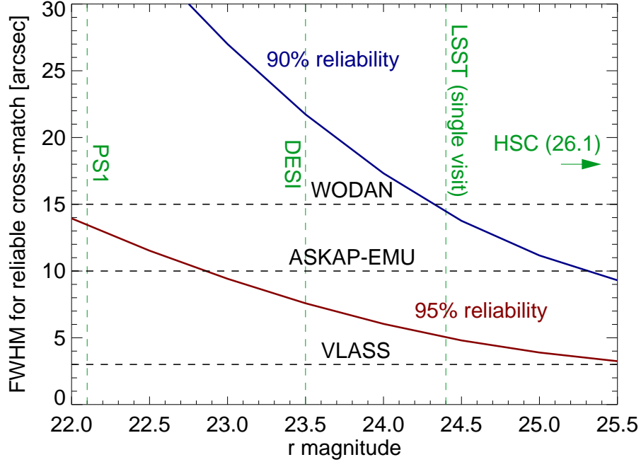
Figure 5: FWHM resolution required to achieve reliable cross-matches at fainter magnitudes using r -band galaxy counts from the CFHTLS-D1 1 \text{ deg}^2 survey (Jarvis, private communication). Two curves are shown for 90% and 95% reliable identifications, and the resolutions of VLASS, ASKAP-EMU and WODAN are shown. This confirms that the SKA pathfinders are at best marginally sufficient for identifications at SDSS/Pan-STARRS depths, while VLASS is usable all the way to r = 25 .
