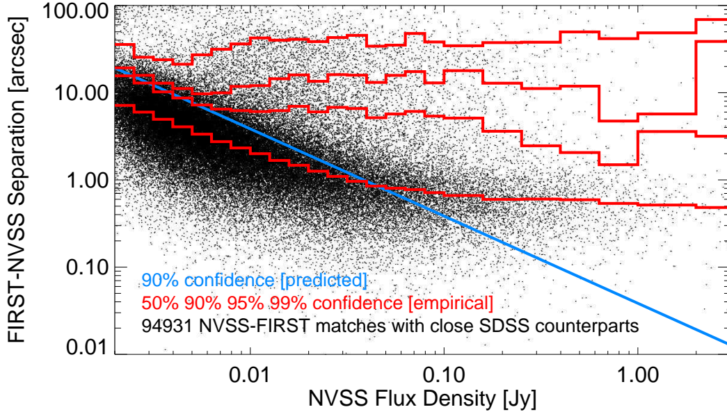
Figure 9: Position difference between NVSS and FIRST positions as a function of NVSS flux density. The sample includes only objects that have a close SDSS counterpart to the FIRST source position (within 0.7'' ). Blue line: Theoretical 90% confidence separation limit computed using the S/N model. Red histograms: (from bottom to top) the 50, 90, 95, and 99% confidence limits, computed by determining the actual separations in each bin. While the 50% curve behaves approximately as expected, the tail of the distribution is clearly non-Gaussian and has many more distant outliers than expected based on the 90% prediction.
