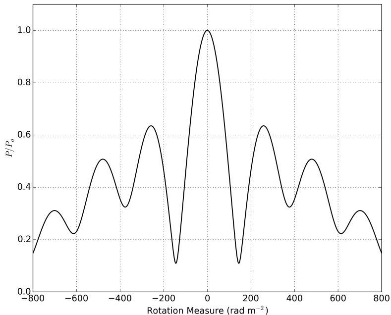
Figure 2: Faraday depth response function. The available non-RFI contaminated frequencies at S-band provides a FWHM response of \sim 200 \text{ rad m}^{-2} .
