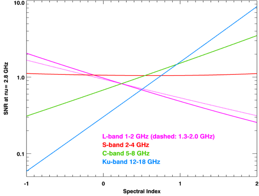
Figure 4: Signal-to-noise ratio sensitivity as a function of spectral index. The figure considers a source with a fixed signal-to-noise ratio (SNR) at a frequency of 2.8 GHz (S band), normalizing sensitivity to it. Higher signal-to-noise ratios can be obtained for non-thermal sources (spectral index < 0 ) by observing at lower frequencies (L band, pink solid and dashed lines) at the cost of lower sensitivity to thermal sources (spectral index \gtrsim 1 ). Conversely, higher signal-to-noise ratios can be obtained for thermal sources at higher frequencies (C band, green solid line; Ku band, blue solid line) at the cost of lower sensitivity to non-thermal sources. The Galactic radio source population contains both thermal and non-thermal emitters, and the 2–4 GHz observing frequency range for the VLASS provides a balance in the sensitivity for these two classes of sources.
