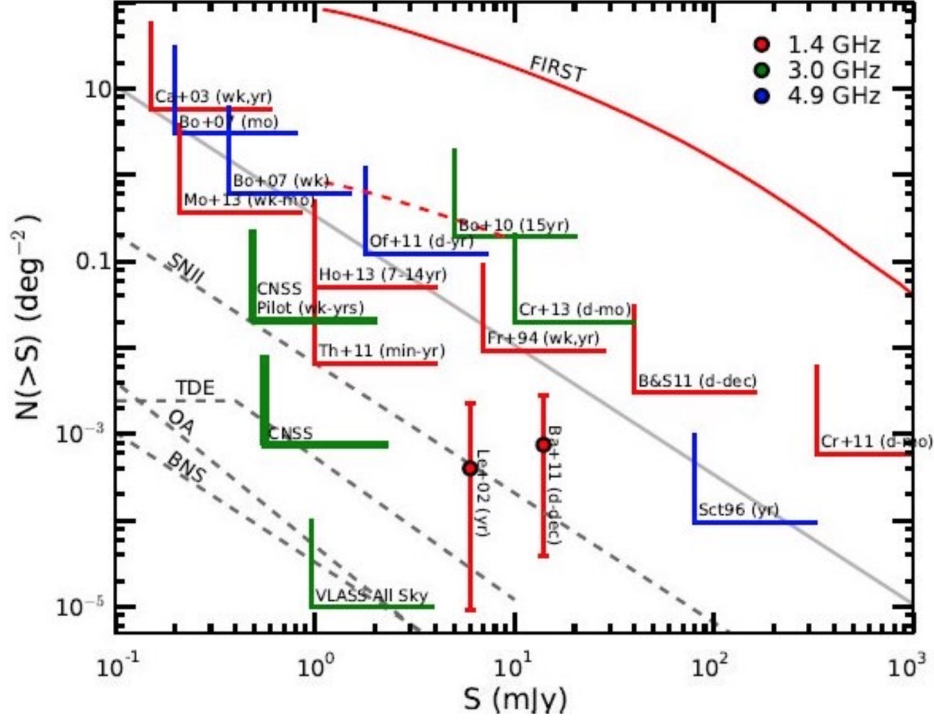
Figure 1: The phase space of explosive extragalactic radio transients. The dashed black lines give the instantaneous source counts for different classes of transients at 3 GHz. The rates for Type II supernovae, neutron star mergers (NS-NS), tidal disruption events (referred to as Swift J1644-like) and for highly luminous supernovae such as SN1998bw are from Frail et al. (2012) and those for orphan long-GRB afterglows are from Ghirlanda et al. (2014). The dashed red line denotes the variable extragalactic source population [1% of the persistent sources; (e.g., Mooley et al., 2013) and references therein]. The solid red line represents extragalactic source counts from FIRST. The dashed grey line is the transient rate claimed by Bower et al. (2007). Wedges indicate upper limits to the transient rates from previous surveys, and errorbars ( 2\sigma ) are transient rates for past detections. The markers are color-coded according to observing frequency. The limits shown for the VLASS represent the expected cumulative number of detected transients, with the requirement that a transient event must be detected at > 10\sigma in a single epoch, to overcome thermal noise fluctuations in the data when comparing 2 epochs ( > 10^{11} synthesized beams per epoch) as well as image artifacts that masquerade as transients. We note that this is conservative - one can use much lower detection threshold (e.g. 6\sigma ) combined with the requirement that the detected transient must be located in a nearby galaxy ( z < 0.1 ) to overcome high- \sigma thermal noise fluctuations. This alone would increase the detection yield for extragalactic transients by an order of magnitude. It is crucial to emphasize that these rates represents the mean number density of such transient sources at any given time, but the identification of a source as a transient can only be best realized with a reference image taken prior the explosive event. The required separation between reference and detection image depends strongly on frequency, with the mean time to maximum brightness for radio supernovae, for example, varying from weeks at 20 GHz to > 2 years at 1.4 GHz. Thus, to maximize detection sensitivity to transients on all timescales, both short and long, epochs should be separated by gaps greater than the mean time to maximum brightness for all classes transients. This is the strategy adopted by the VLASS, with epochs spaced by 32 months, and is reflected in the calculated rates.
