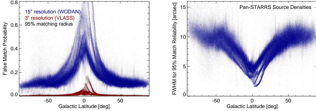
Figure 10: Left: Probability of a false match in Pan-STARRS as a function of Galactic latitude. The actual density of PS1 objects was used to calculate the likelihood of a false counterpart within the 95% confidence radius. The plot shows probabilities both for the WODAN 15'' resolution (blue) and VLASS S-band 3'' resolution (red). Over most of the extragalactic sky \sim 10\% of WODAN-PS1 cross-matches will be chance coincidences, compared with < 1\% of VLASS-PS1 matches. VLASS positions are sufficient for reliable identifications even close to the Galactic plane. Right: FWHM resolution required to achieve 95% cross-match reliability in Pan-STARRS as a function of Galactic latitude. In the extragalactic sky ( |\delta| > 30^\circ ) a resolution better than 10'' is required. WODAN does not have the required resolution; ASKAP-EMU just reaches this limit but will not cover most of the northern sky. The VLASS S-band survey easily meets this requirement.
