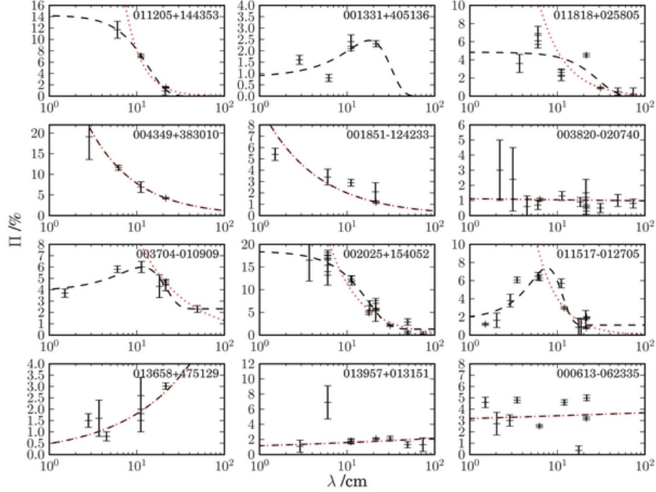
Figure 3: Broad-band spectrum of percent polarization for a sample of radio sources from Farnes et al. (2014a). The diverse complex spectra arise from a combination of internal Faraday depolarization effects (at longer wavelengths) and intrinsic magnetic properties (at shorter wavelengths).
