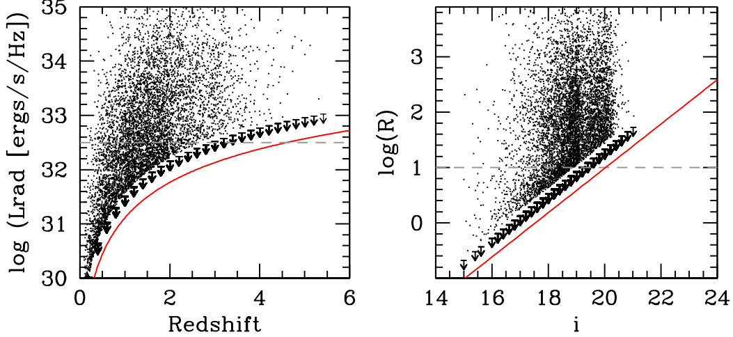
Figure 6: Left: Radio luminosity plotted against redshift for SDSS quasars. The dashed line indicates a division between radio- loud and radio-quiet quasars according to the radio luminosity (e.g., Goldschmidt et al., 1999). Radio upper limits are shown by arrows (offset downward slightly from the actual limits and sparse sampled for clarity). The depth of the VLASS (as indicated by the red line) allows us to push the redshift limit of radio-loud completeness from z = 2.7 to z > 4 . Right: Radio loudness (as measured by the ratio of radio to optical flux) vs. i -band magnitude. The dashed line shows the traditional division between radio-loud and radio-quiet quasars of \log(R)=1 . Upper limits are given as arrows (offset downwards slightly and for clarity). The solid red line shows the improvement that results from VLASS. Not only will we be complete to radio-loud quasars to i = 19.9 , combining with the deep optical data will allow us to study the most radio-loud objects to i \sim 24 over a significant fraction ( \sim 30\% ) of the sky.
