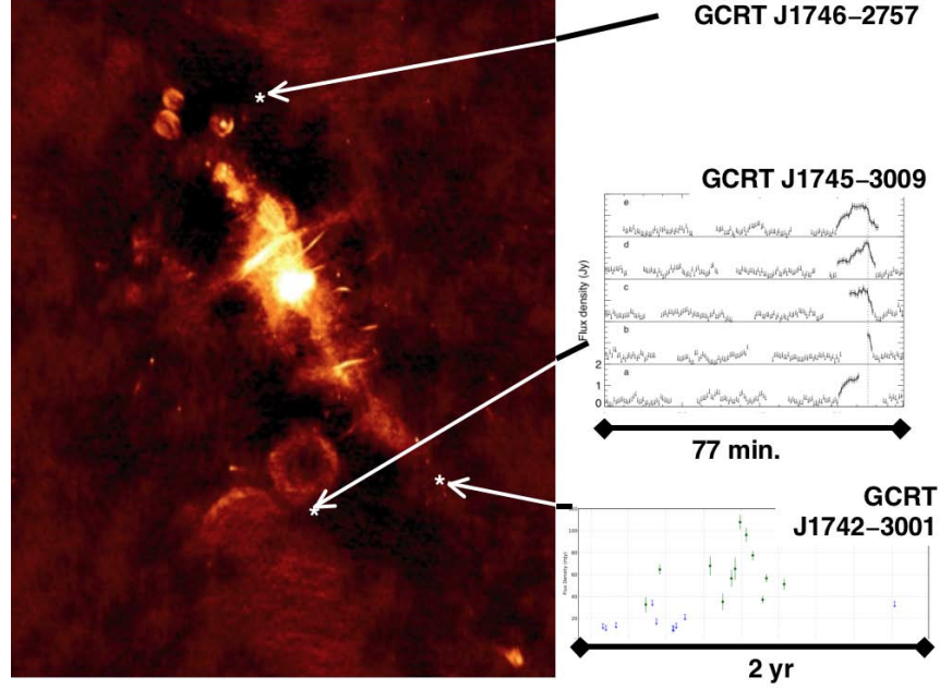
Figure 8: The diversity of the light curves for transients toward the Galactic center Hyman et al. (2002, 2005, 2009). The transient GCRT J1745–3009 burst several times (duration \sim 10 minutes) during a 6-hr observation, with subsequent bursts detected over the next 1.5 yr; GCRT J1742–3001 brightened and faded over several months, preceded 6 months earlier by intermittent bursts; and GCRT J1746–2757 was detected in only a single epoch. None of these objects has been identified nor has a multi-wavelength counterpart been found. The background image is the Galactic center at 330 MHz. Figure taken from Lazio et al. (2009).
