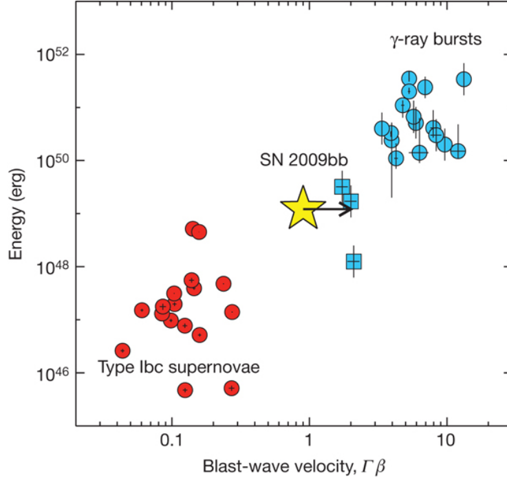
Figure 7: Kinetic energy in the fastest moving ejecta is plotted against shock wave speeds and compared for SNe and GRBs. It can be seen that the normal supernova shock wave carries a few orders of magnitude less energy than a GRB shock wave. Similar to the velocity space, the energy distribution of SN and GRBs also appear bimodal. Events similar to SN 2009bb populating this parameter space remain to be discovered (Margutti et al. (2013a); Soderberg et al. (2010)).
