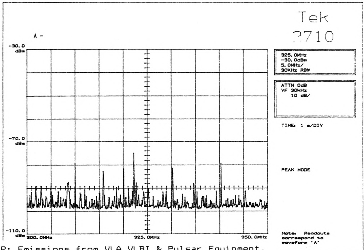
FIGURE 2: TOP: Emissions from VLA VLBI & Pulsar Equipment. BOTTOM: Background Emissions from Other Equip.
