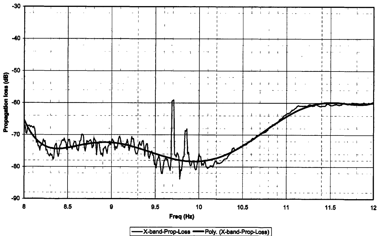
X-band: Vertex-room-to-LNA-input, propagation loss: 20080429 test data
