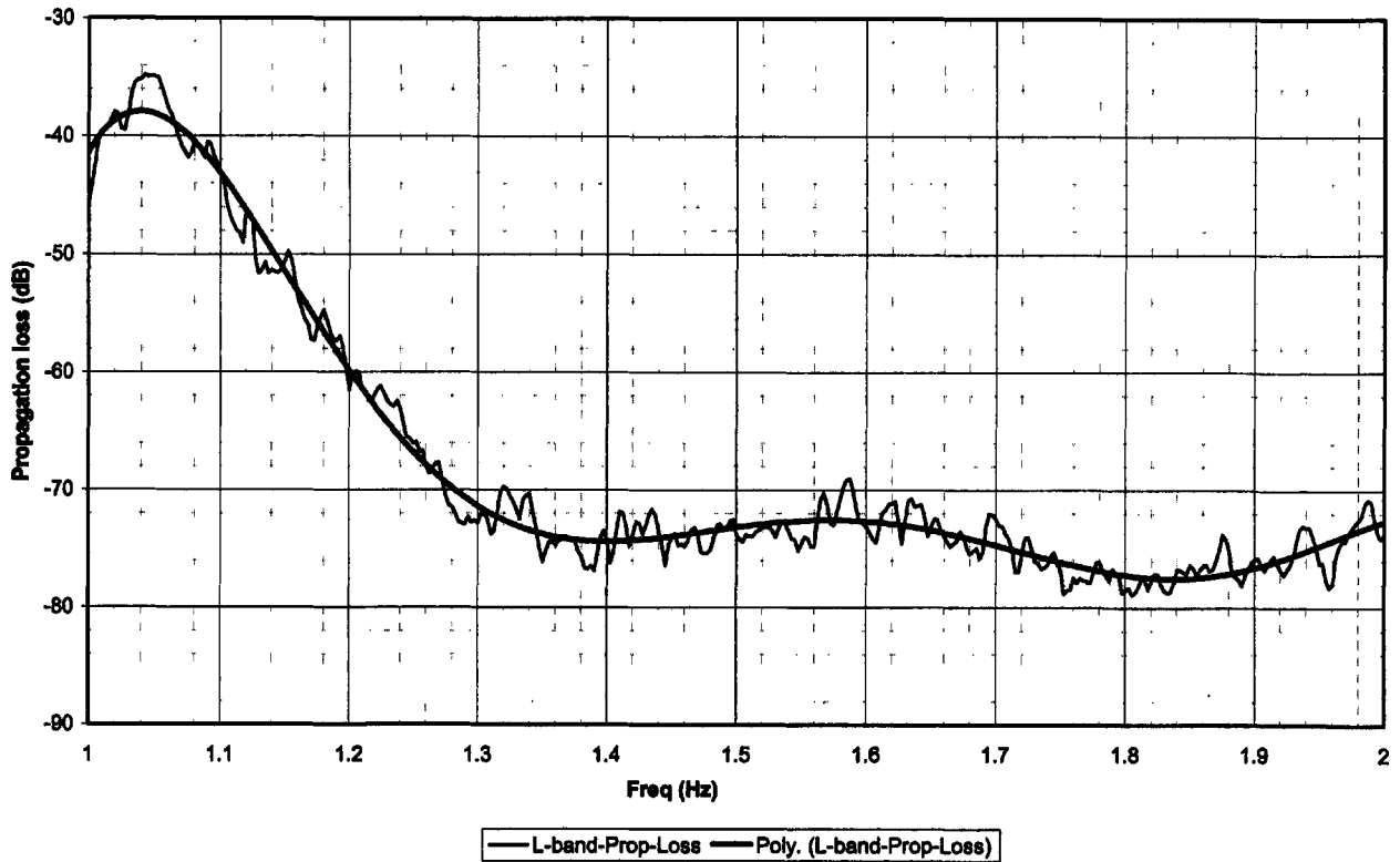
L-band: Vertex-room-to-LNA-input, propagation loss: 20080429 test data
