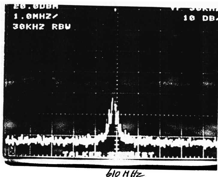
Fig. 7- Spectra taken at IF CONVERTER FP BNC (IF MONITOR). See figure 6 for the test set.
