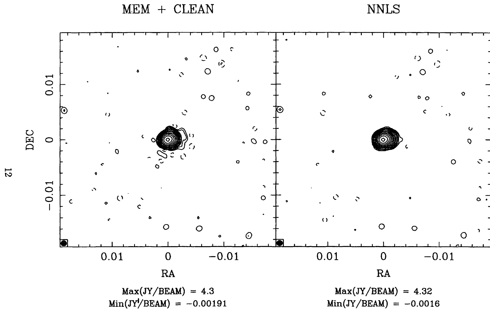
Figure 4: Superresolution. The left panel is produced with combination of MEM and CLEAN, the right with NNLS.
