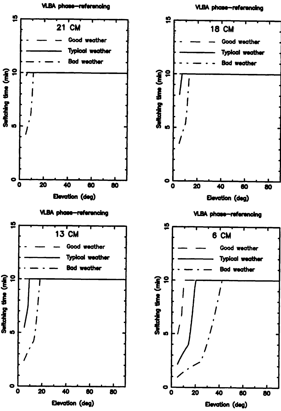
Figure 4: Maximum phase-referencing switching times for good, typical, and bad weather, for wavelengths ranging from 6 cm to 21 cm.
