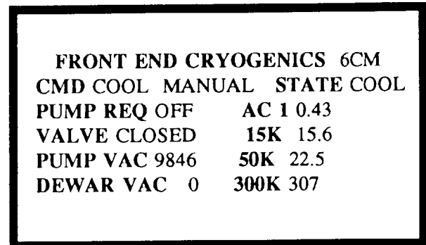
Figure 6 VLBA F105 Cryogenics Screen
