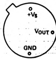
TO-5 BOTTOM VIEW
