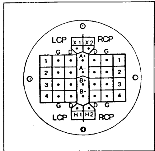
Figure 4 DC Feedthrough
