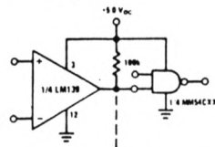
Driving CMOS
