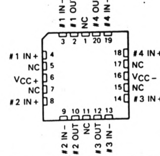
TL084M . . . FK CHIP CARRIER PACKAGE (TOP VIEW)
