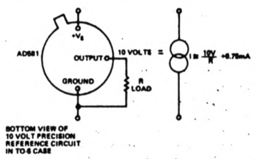
Figure 11. A Two-Terminal Precision Current Limiter
