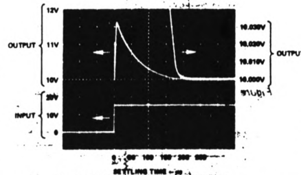
Figure 6. Output Settling Characteristics
