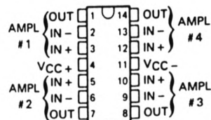
TL084, TL084A, TL084B D, J, OR N PACKAGE (TOP VIEW)
