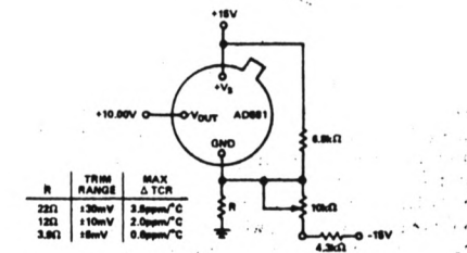
Figure 2. Optional Fine Trim Configuration
