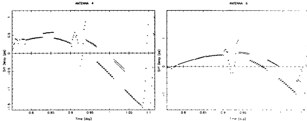
Figure 8: Difference between the CL table geodelay values from the processing pass done with good EOP and the geodelay plus the CLCOR correction for the pass done with poor EOP. The left plot is for Kitt Peak and the right plot is for Mauna Kea. If the CLCOR corrections were perfect, the difference would be zero. Note that 1 ps at 8.4 GHz is 0.0084 turn of phase or about 3 degrees of phase, so the differences are small.
