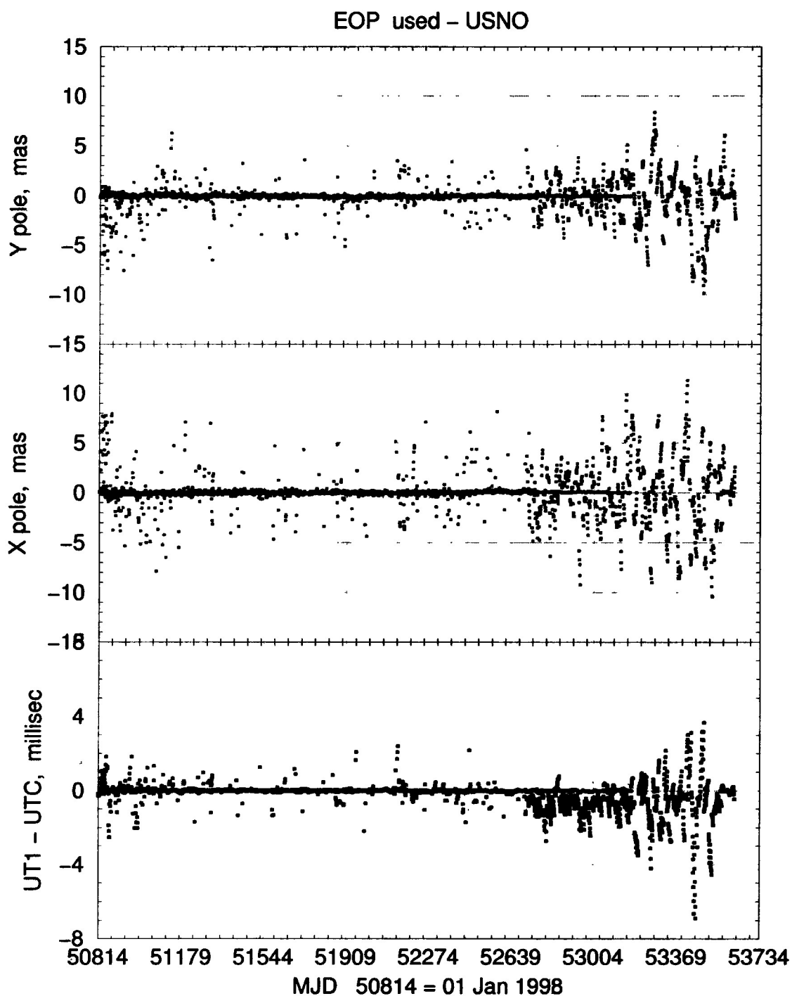
Figure 1: Plot of the offsets between the EOP parameters used in correlator jobs and reference good EOP values from a usno_finals.erp file. Data are shown for times since 1998. Vertical bars mark the year boundaries with the last partial year being 2005. The correlator jobs began to include poor EOP in May 2003 and were corrected in August 2005 just before the last data shown here. Longer range predicted EOP values started being used in June 2004, accounting for the worsening of the offsets at that time.
