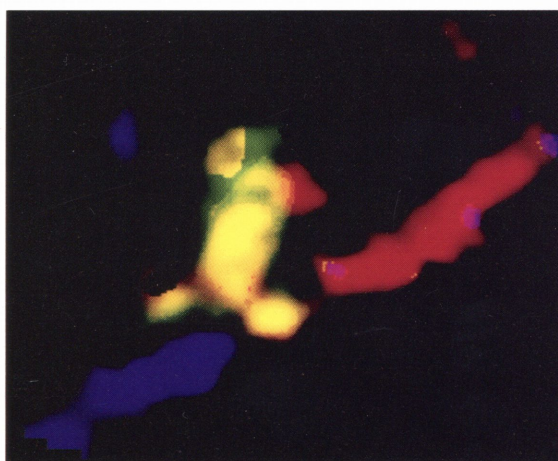
The first light of a newborn star (yellow) expels gas toward (blue) and away (red) from us.
