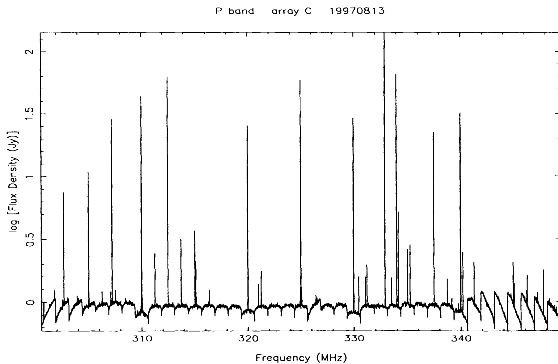
Figure 4: Typical P-band interference spectrum with 6 kHz resolution.
